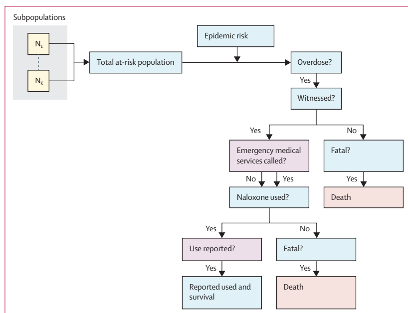
Figure 1: Simplified model overview of fatal and non-fatal opioid overdose with naloxone use by US state Diagram indicates where data are captured in the model (non-blue boxes) with other latent branches suppressed. The at-risk population is stratified by risk type ( N_1 to N_k ), which are combined together to produce an effective population size of individuals at risk of an opioid overdose. A per-month rate of opioid overdose is dependent on epidemic type and underlying circulation of fentanyl and its derivatives (indicated by the epidemic risk box). Each estimated opioid overdose is then entered into a decision tree to determine the probability of the opioid overdose resulting in death, whether there is a reported use of naloxone, or neither. Whether an opioid overdose is fatal is dependent on whether it is witnessed, whether emergency medical services were called, whether naloxone is used, and the underlying risk of death for an intervened overdose. The probability of naloxone use is dependent on whether an overdose is witnessed, naloxone is available and used by a witness, and whether its use is reported.
